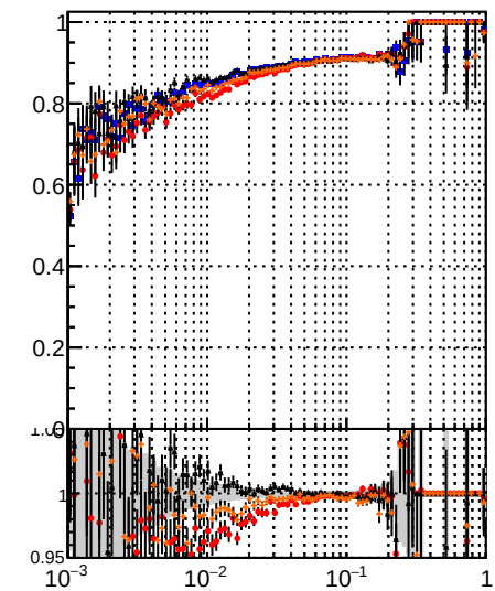
Fake rate vs DQM Displaced SUSY CKE CKEfit BDT DQM Displaced SUSY CKEfit BDT
