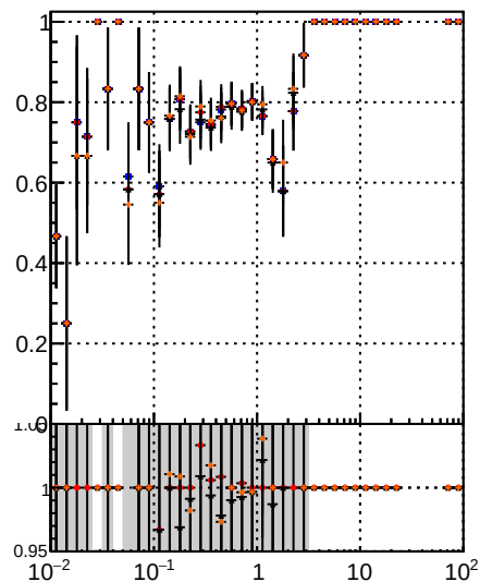
Fake rate vs v DOM Displaced SUSY CKFit BDT DOM Displaced SUSY CKFit BDT DOM Displaced SUSY CKFit BDT
