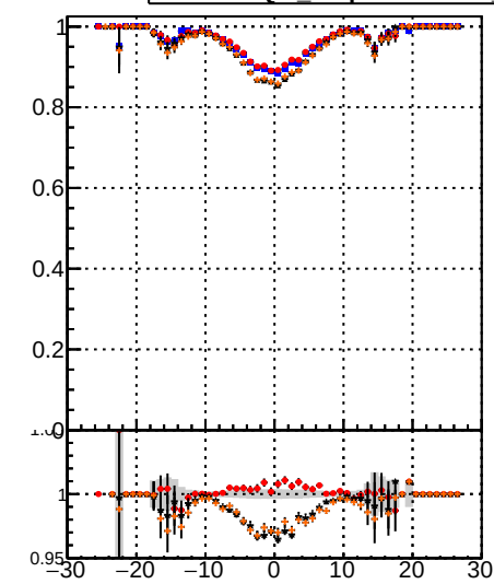
—●— BQM Displaced SUSY CKE —●— BQM Displaced SUSY CKEfit —●— BQM Displaced SUSY BDT —●— BQM Displaced SUSY mkFit
