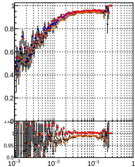
Fake rate vs DQM Displaced SUSY CKEfit DQM Displaced SUSY CKEfit BDT DQM Displaced SUSY CKEfit DQM Displaced SUSY mkFit BDT
