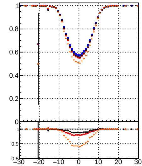
DOM Displaced SUSY CKE DOM Displaced SUSY CKE fit DOM Displaced SUSY mkFit DOM Displaced SUSY BDT
