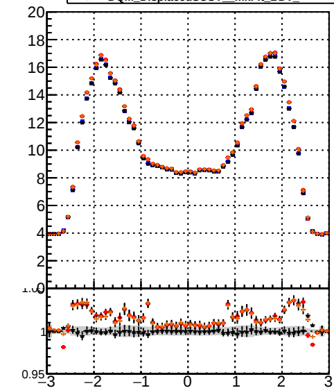
mean hit Legend: Blue line: DQM_DisplacedSUSY_CKF Red line: DQM_DisplacedSUSY_mkFit Black line: DQM_DisplacedSUSY_CKF_BDT Orange line: DQM_DisplacedSUSY_mkFit_BDT
