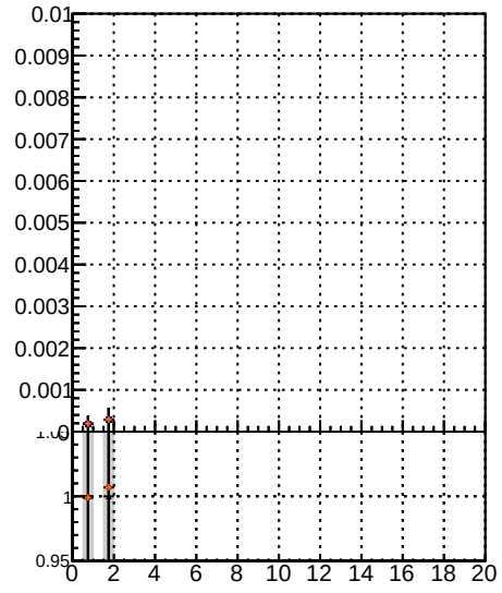
Fake rate vs. BSM Displaced SUSY CKFit BSM Displaced SUSY CKFit BDT BSM Displaced SUSY CKFit BDT
