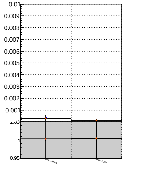
Fake rate vs. BSM Displaced SUSY CKFit BSM Displaced SUSY CKFit BDT BSM Displaced SUSY CKFit BDT
