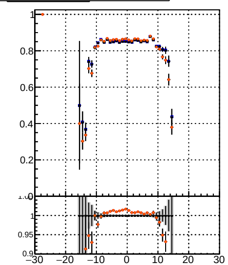
Fake rate vs d Legend: BSM Displaced SUSY (blue circles), BSM Displaced SUSY CKFit (black circles), BSM Displaced SUSY CKFit BDT (orange circles)
