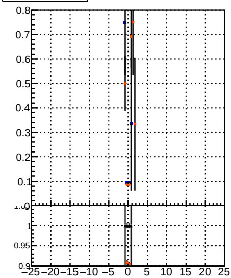
Fake rate vs d Legend: BSM Displaced SUSY (blue circles), BSM Displaced SUSY CKFit (black circles), BSM Displaced SUSY CKFit BDT (orange circles)
