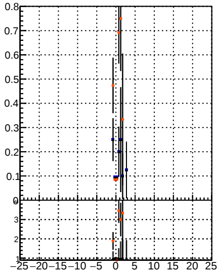
Fake rate vs d Legend: BSM Displaced SUSY CKFit BSM Displaced SUSY CKFit BDT BSM Displaced SUSY CKFit BDT
