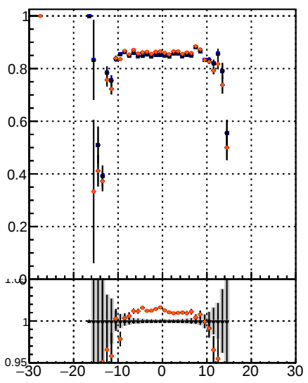
Fake rate vs d Legend: BSM Displaced SUSY CKFit BSM Displaced SUSY CKFit BDT BSM Displaced SUSY CKFit BDT
