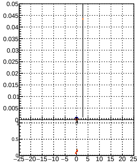
Duplicates Rate vs \Delta xy
