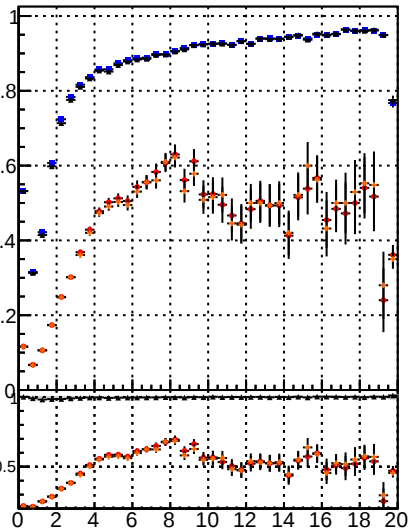
Fake rate vs. \chi^2 Legend: BDT Displaced SUSY CKFit BDT
