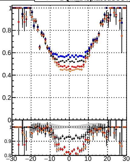
DOM Displaced SUSY CKE DOM Displaced SUSY CKEfit DOM Displaced SUSY CKEfit BDT DOM Displaced SUSY mktfit BDT
