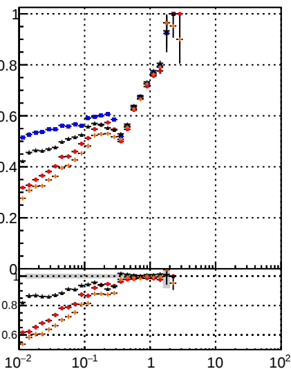
DOM Displaced SUSY CKE DOM Displaced SUSY CKEfit DOM Displaced SUSY CKEfit BDT DOM Displaced SUSY mktfit BDT
