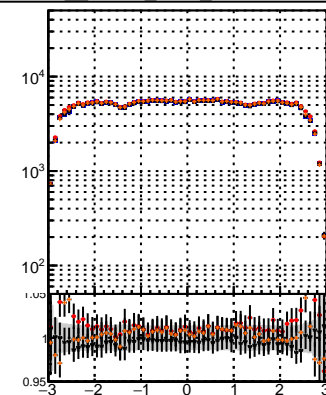
SUSY → CKFit SUSY → CKFit SUSY → CKFit SUSY → CKFit
