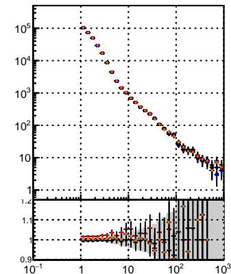
SUSY → CKFit SUSY → CKFit SUSY → CKFit SUSY → CKFit
