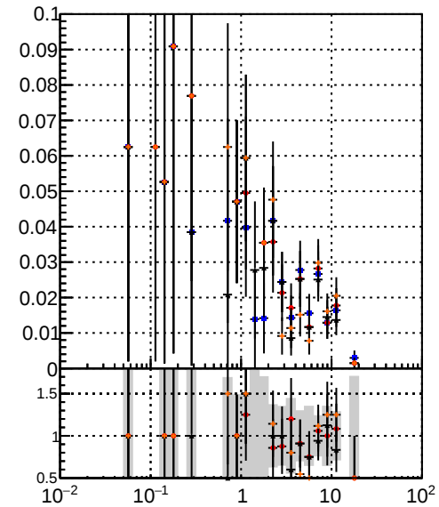
Efficiency vs vertpos DQM_DisplacedSUSY_CKF DQM_DisplacedSUSY_mkFit DQM_DisplacedSUSY_CKF_BDT DQM_DisplacedSUSY_mkFit_BDT
