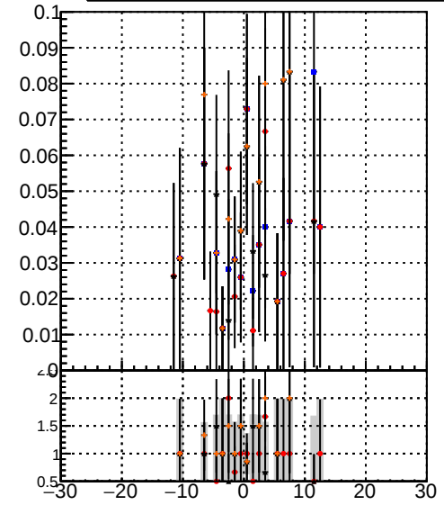
Efficiency vs vertpos DQM_DisplacedSUSY_CKF DQM_DisplacedSUSY_mkFit DQM_DisplacedSUSY_CKF_BDT DQM_DisplacedSUSY_mkFit_BDT
