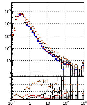
N of reco track vs energy DOM Displaced SUSY GKE BDT fit BDT fit BDT fit BDT fit Energy [GeV]
