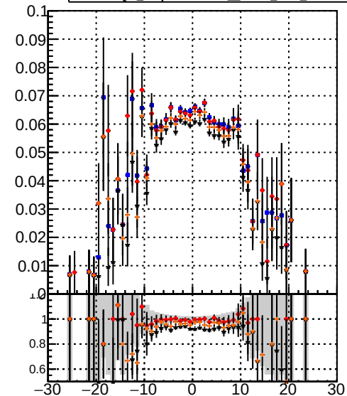
Efficiency vs. sim PV z —●— DQM_DisplacedSUSY_CKF —●— DQM_DisplacedSUSY_mkFit —●— DQM_DisplacedSUSY_CKF_BDT —●— DQM_DisplacedSUSY_mkFit_BDT
