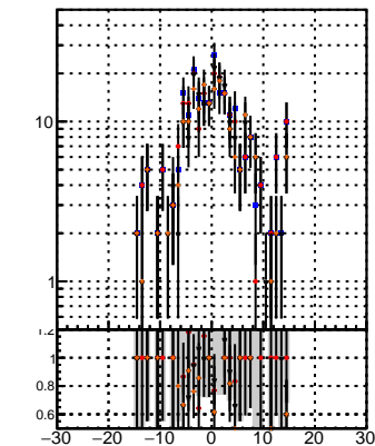
N of associated (recoToSim) loopers tracks vs dz
