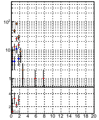
● BDM ● Displaced SUSY ● GKE — BDM — Displaced SUSY — GKE + BDT + WRFIT
