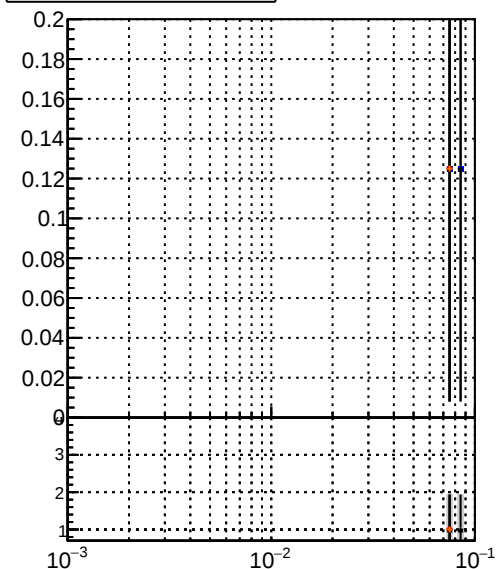
Efficiency vs \Delta R (track, jet)
