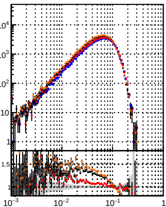
N of reconstructed tracks vs dR
