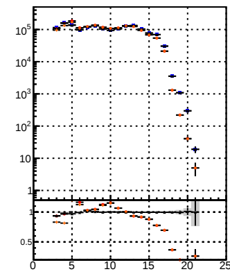
DOM Displaced SUSY CKE DOM Displaced SUSY mkt-fit BDT DOM Displaced SUSY mkt-fit BDT
