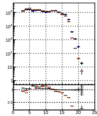
DOM Displaced SUSY CKE DOM Displaced SUSY mkt-fit BDT DOM Displaced SUSY mkt-fit BDT
