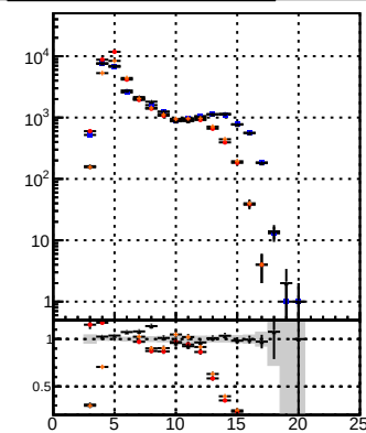
edSUSY—mktFit BDT
