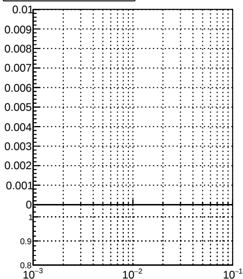
Efficiency vs d_r(\text{track, jet})
