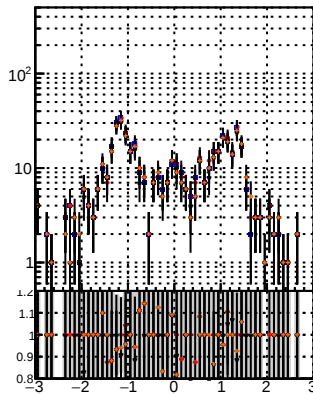
N of reco track vs \eta BQM Displaced SUSY GKF-it BDT BQM Displaced SUSY GKF-it BDT \eta eta
