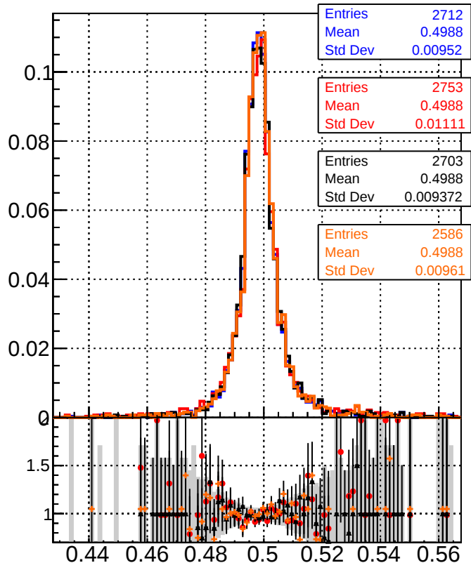
Mass of good reco K0S
