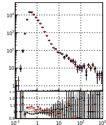
N of reco track vs energy DOM Displaced SUSY GKE BDT fit BDT
