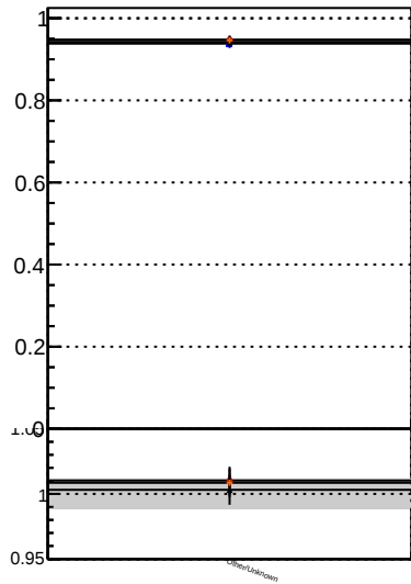
Fake rate vs. BSM Displaced SUSY CKFit BDT BSM Displaced SUSY CKFit BDT
