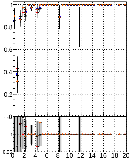
Fake rate vs. BSM Displaced SUSY CKFit BDT BSM Displaced SUSY CKFit BDT
