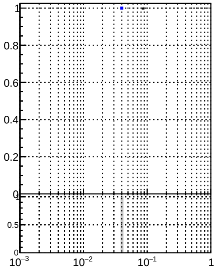
Fake rate vs \sqrt{s} DOM Displaced SUSY CKE BDT Fake rate vs \sqrt{s} DOM Displaced SUSY CKE BDT Fake rate vs \sqrt{s} DOM Displaced SUSY CKE BDT
