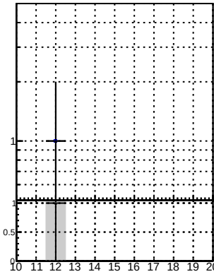
N of associated (recoToSim) tracks vs hit
