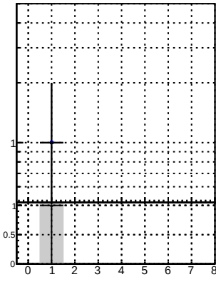
N of associated (recoToSim) tracks vs pixellayer
