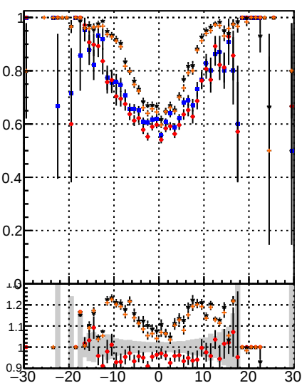
Fake rate vs d DOM Displaced SUSY GKE DOM Displaced SUSY GKE mkt BDT mkt
