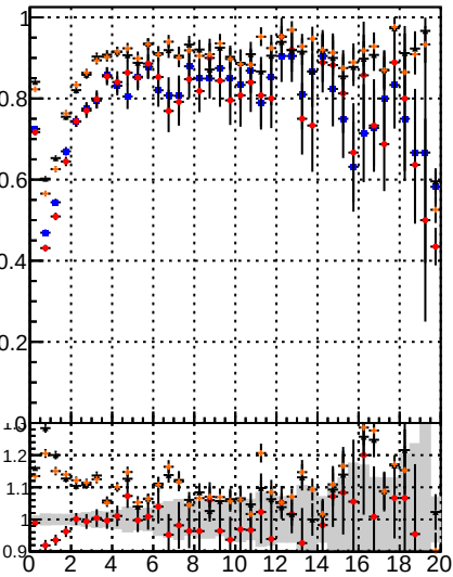
Fake rate vs. BDM Displaced SUSY CKFit BDT BDM Displaced SUSY CKFit BDT
