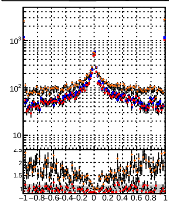
—●— DOM Displaced SUSY CKE —●— DOM Displaced SUSY CKE it BDT —●— DOM Displaced SUSY mkt it BDT
