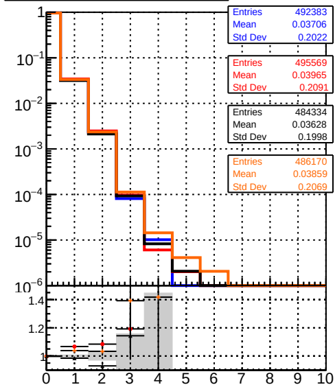
mean hit Legend: DQM_DisplacedSUSY CKF, DQM_DisplacedSUSY mkFit, DQM_DisplacedSUSY CKF_BDT, DQM_DisplacedSUSY mkFit_BDT
