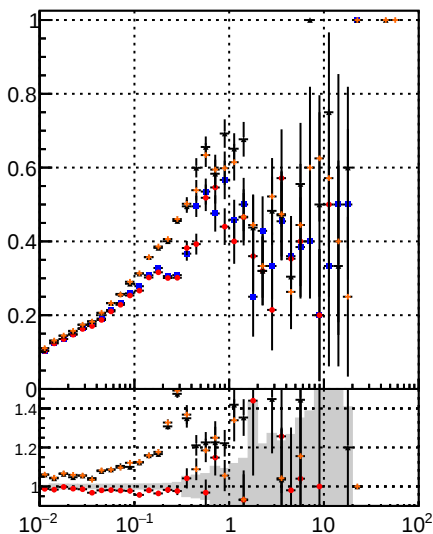
Fake rate vs \sqrt{s} \sqrt{s} DOM Displaced SUSY CKE DOM Displaced SUSY mktFit DOM Displaced SUSY CKE mktFit DOM Displaced SUSY CKE mktFit BDT 0 0.0 0.0 0.0 0.0 2 0.0 0.0 0.0 0.0 4 0.0 0.0 0.0 0.0 6 0.0 0.0 0.0 0.0 8 0.0 0.0 0.0 0.0 10 0.0 0.0 0.0 0.0 12 0.0 0.0 0.0 0.0 14 0.0 0.0 0.0 0.0
