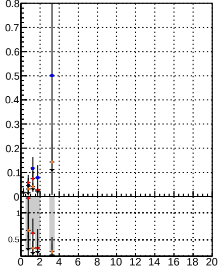
Fake rate vs. \chi^2 for BSM Displaced SUSY CKFit BDT
