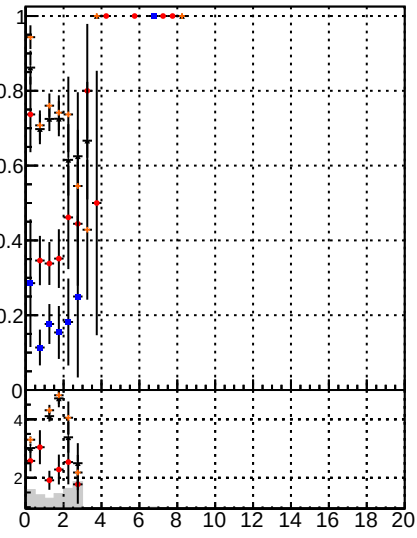
Fake rate vs. \chi^2 for BSM Displaced SUSY CKFit BDT
