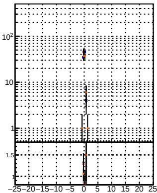
—●— DOM Displaced SUSY CKE —●— DOM Displaced SUSY CKE it —●— DOM Displaced SUSY mke it BDT —●— DOM Displaced SUSY mke it BDT
