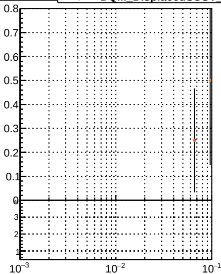
Fake rate vs \mu DOM Displaced SUSY CKE DOM Displaced SUSY CKE fit DOM Displaced SUSY mkt fit BDT
