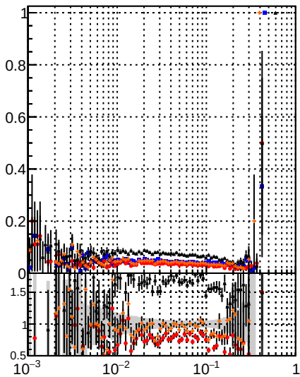
Fake rate vs \mu DOM Displaced SUSY CKE DOM Displaced SUSY CKE fit DOM Displaced SUSY mkt fit BDT
