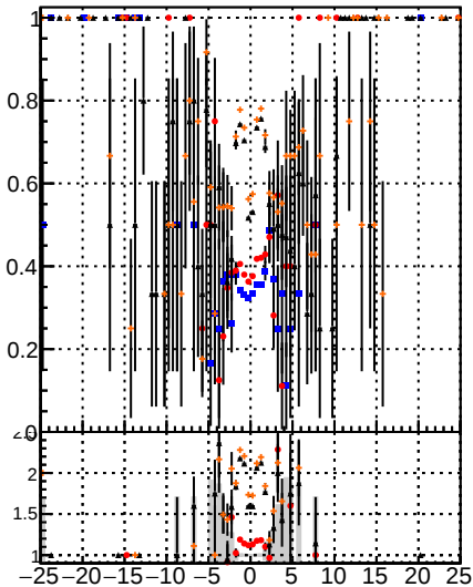
Fake rate vs d —●— DGM Displaced SUSY CKFit —●— DGM Displaced SUSY CKFit BDT —●— DGM Displaced SUSY CKFit BDT
