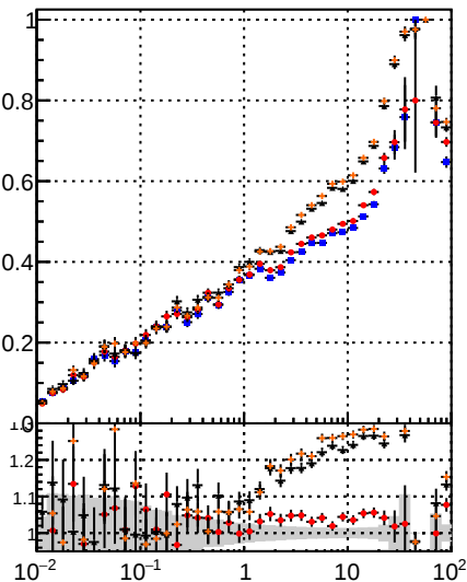
DOM Displaced SUSY CKEfit DOM Displaced SUSY CKEfit DOM Displaced SUSY mktfit BDT
