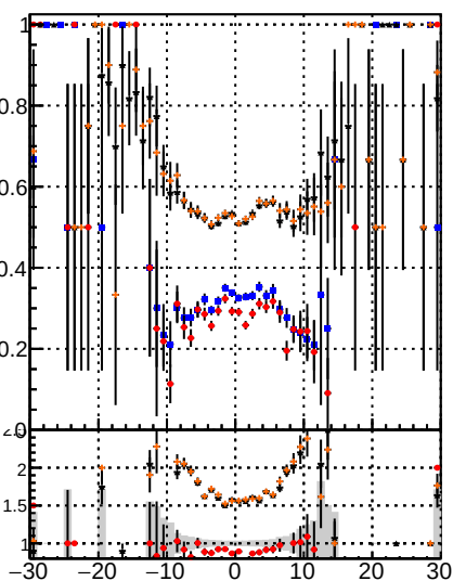
Fake rate vs d —●— DGM Displaced SUSY CKFit —●— DGM Displaced SUSY CKFit BDT —●— DGM Displaced SUSY CKFit BDT
