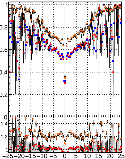
Fake rate vs d —●— BSM Displaced SUSY CKE Fit —●— BSM Displaced SUSY CKE Fit —●— BSM Displaced SUSY CKE Fit —●— BSM Displaced SUSY CKE Fit
