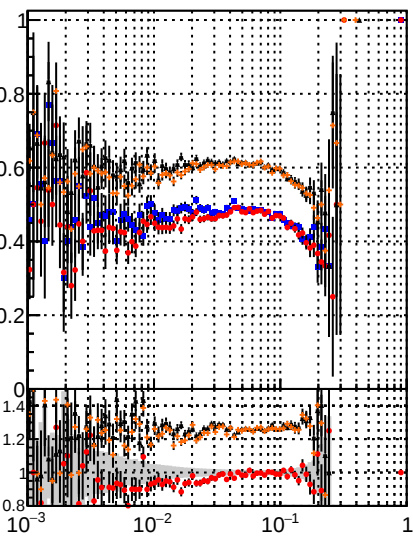
Fake rate vs DQM Displaced SUSY CKE CKEfit BDT DQM Displaced SUSY CKEfit BDT DQM Displaced SUSY mkFit BDT
