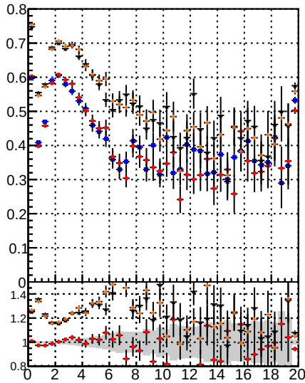
Fake rate vs. BQM Displaced SUSY CKFit CKFit_BDT CKFit_BDT
