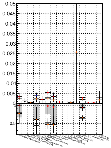
Fake rate vs. BQM Displaced SUSY CKFit CKFit_BDT CKFit_BDT
