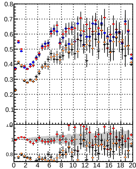
Fake rate vs. BQM Displaced SUSY CKFit CKFit_BDT CKFit_BDT
