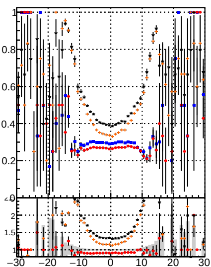
BSM Displaced SUSY CKFit BDT Fake rate vs d
