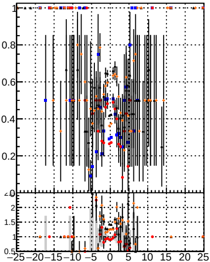
BSM Displaced SUSY CKFit BDT Fake rate vs d
