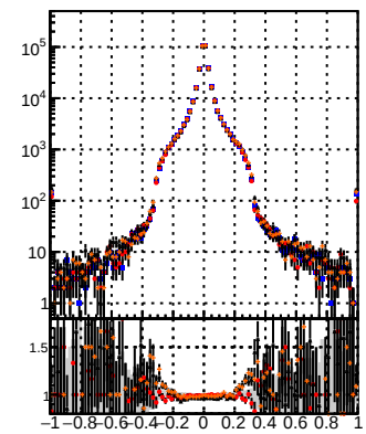
—●— DOM Displaced SUSY CKE —●— DOM Displaced SUSY CKE it —●— DOM Displaced SUSY mke-it BDT —●— DOM Displaced SUSY mke-it BDT
