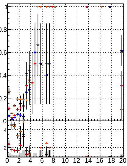
Fake rate vs. BDM Displaced SUSY CKFit BDM Displaced SUSY CKFit_BDT BDM Displaced SUSY CKFit_BDT
