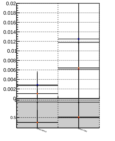
Fake rate vs. BDM Displaced SUSY CKFit BDM Displaced SUSY CKFit_BDT BDM Displaced SUSY CKFit_BDT
