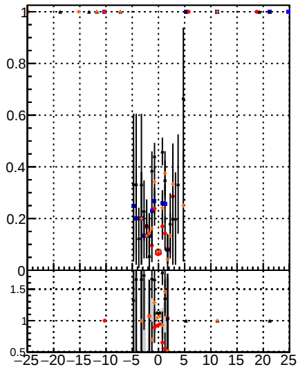
Fake rate vs d —●— BSM Displaced SUSY CKE —●— BSM Displaced SUSY CKE fit —●— BSM Displaced SUSY CKE fit BDT
