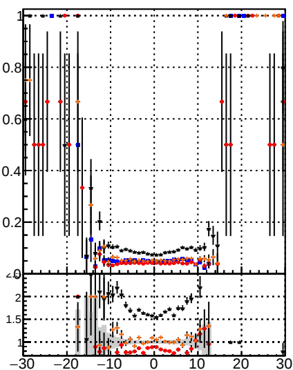
Fake rate vs d DQM Displaced SUSY CKFit DQM Displaced SUSY CKFit BDT DQM Displaced SUSY CKFit BDT
