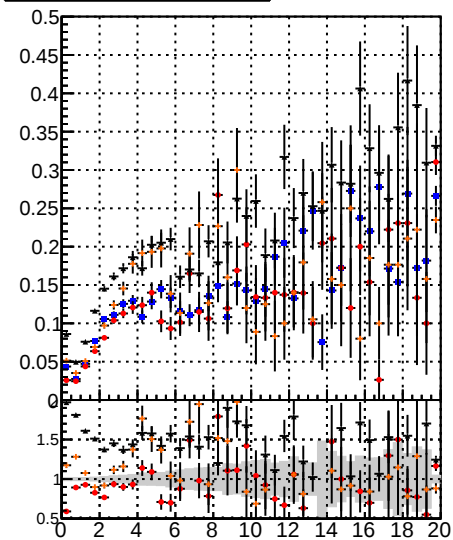
Fake rate vs. BQM Displaced SUSY CKFit BQM Displaced SUSY CKFit BQM Displaced SUSY CKFit
