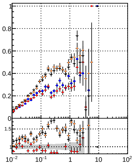
Fake rate vs v DOM Displaced SUSY CKE DOM Displaced SUSY CKEfit DOM Displaced SUSY BDT DOM Displaced SUSY mkFit BDT
